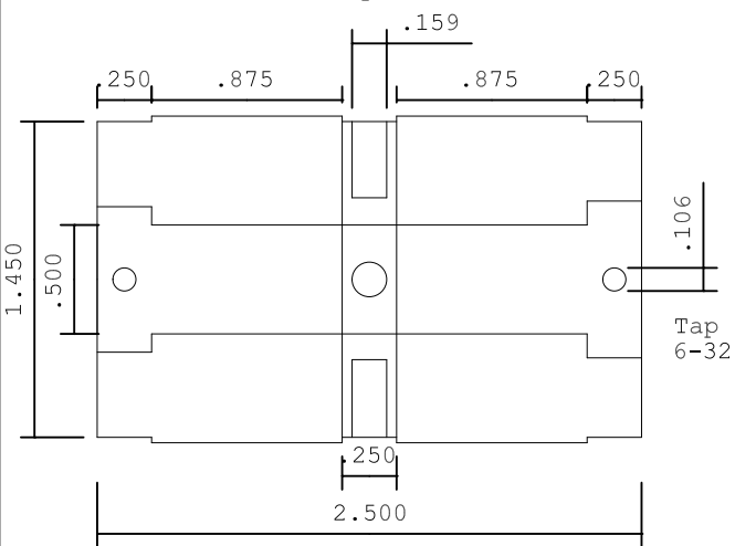
Aluminum Cylinder
