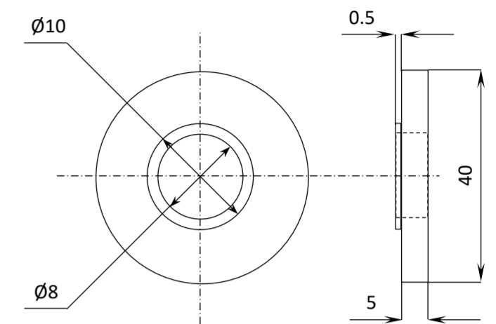
#20 ARM SPIGOT BEARING PLATE
