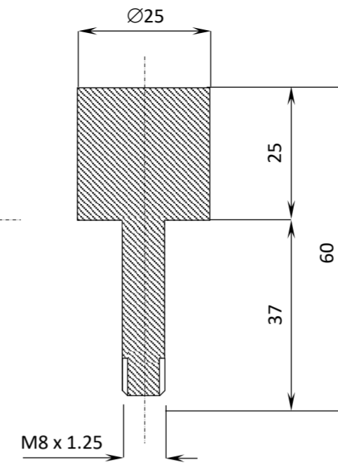
#3 ARM SPIGOT
