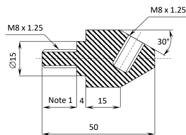
#9 LOCK SCREW BOSS
