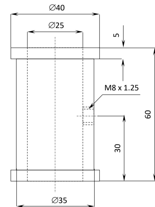
#8 ADJUSTABLE VERTICAL AXIS SUPPORT SLEEVE
