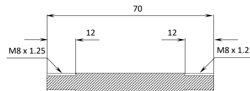
#10 LOCK SCREW HANDLE
