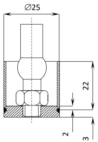
#1 GIMBLE CUP
