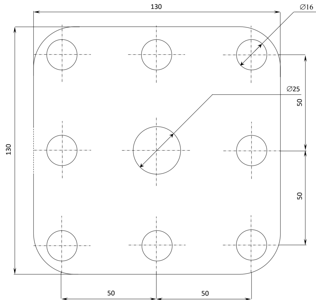
#5 VERTICAL SUPPORT BASE PLATE
