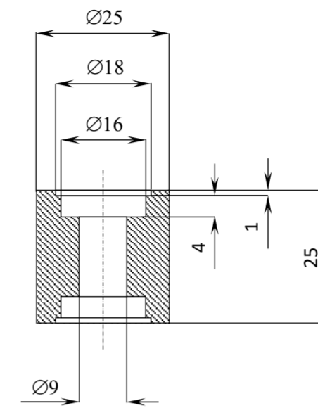
#18 ARM HINGE BEARING CARRIER
