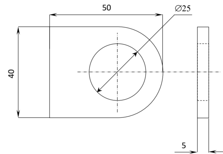
#7 ADJUSTABLE VERTICAL AXIS SUPPORT END PLATE
