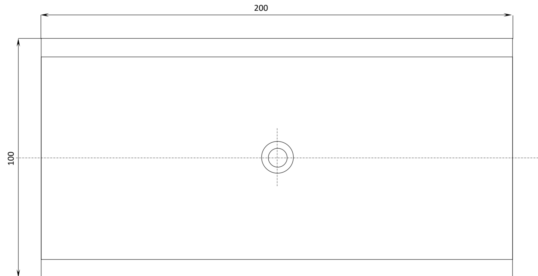
#22 ARM SUPPORT CUP
