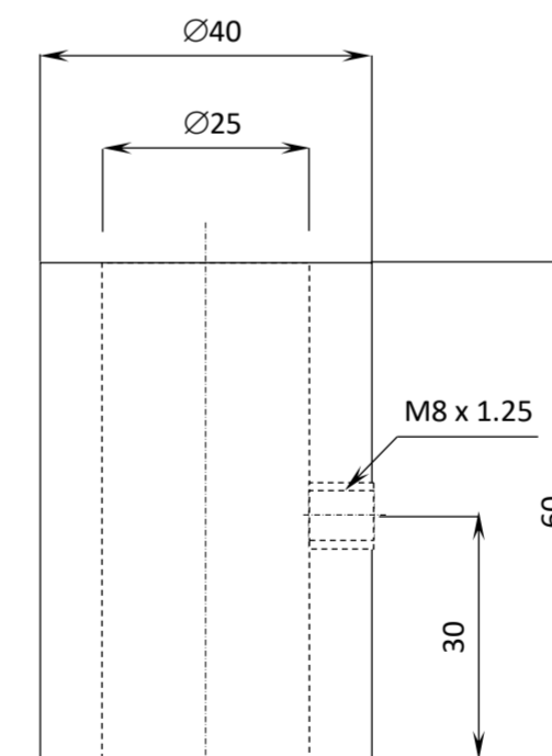
#13 BASE PLATE VERTICAL SUPPORT
