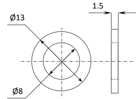
#16 CUSTOM M8 WASHER
