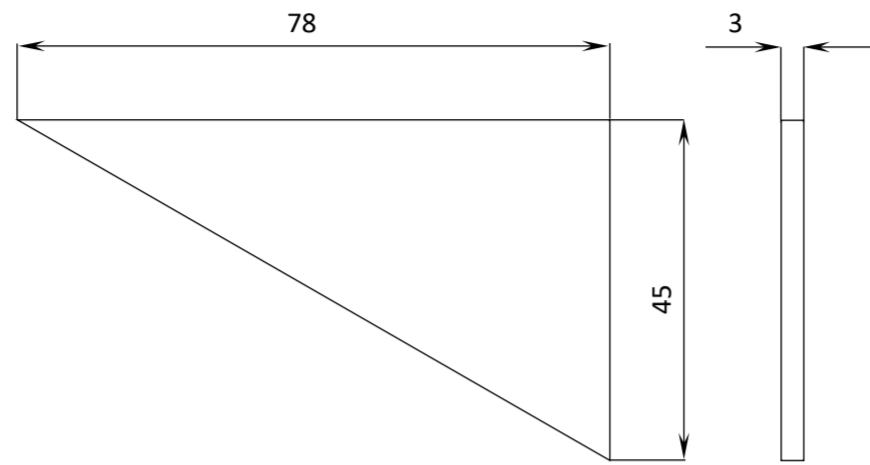
#15 SINGLE HINGED ARM SUPPORT WEB
