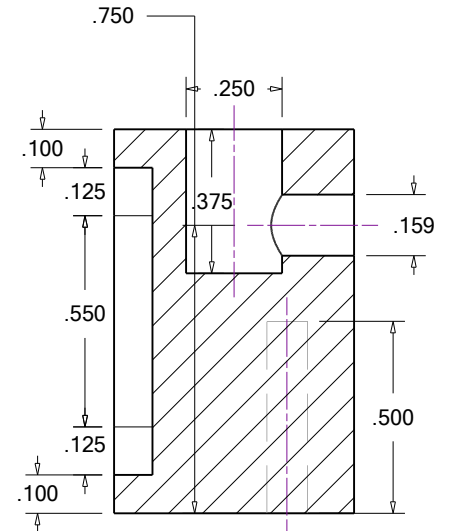
Section B-B
